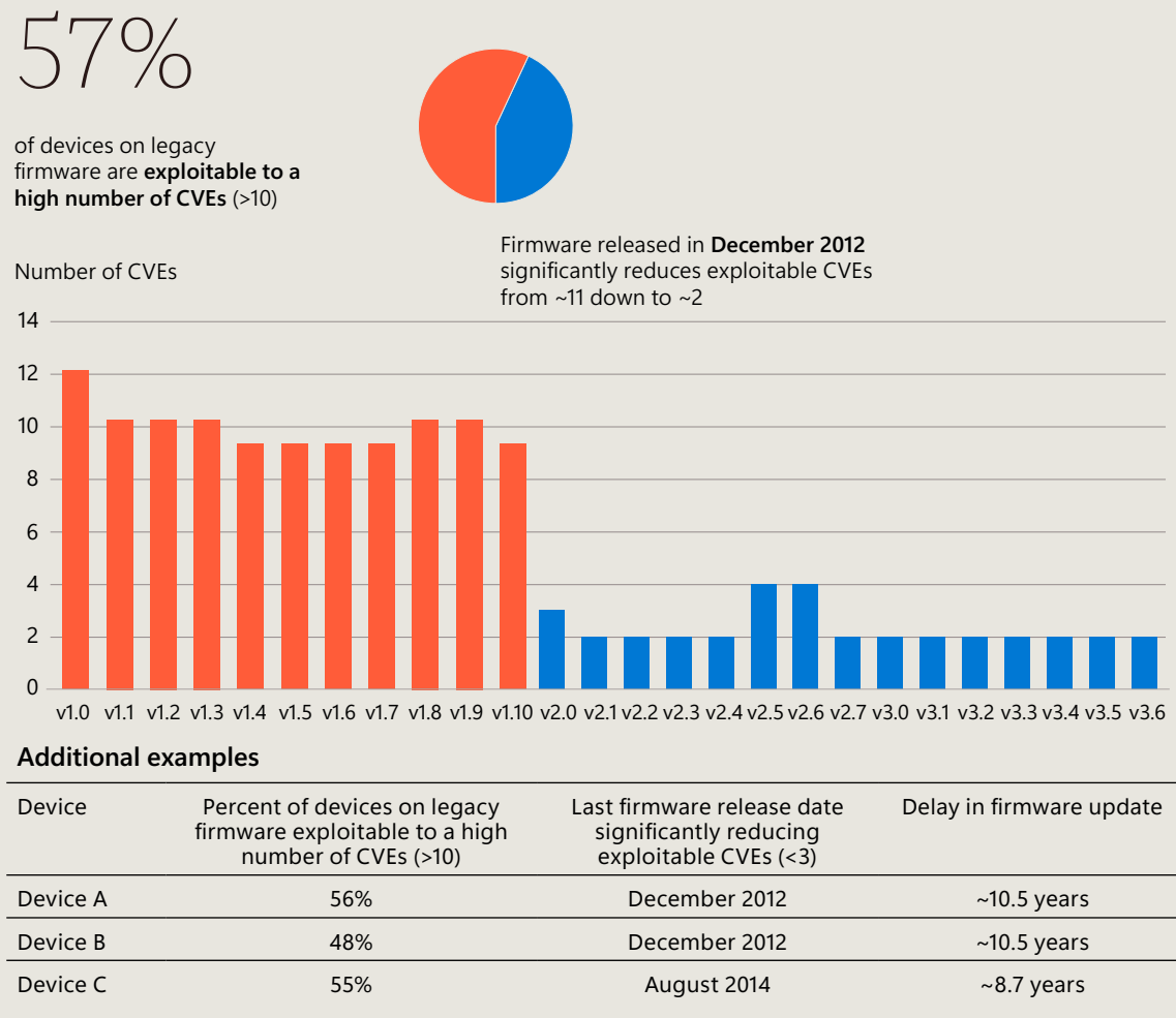
Source: Microsoft Defender for IoT and aDolus Technology
